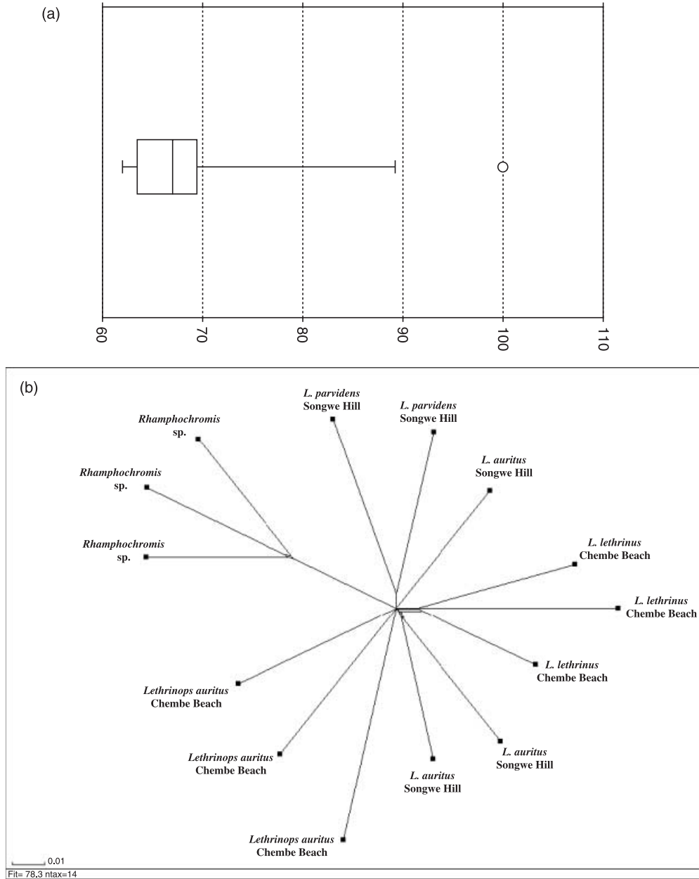
Fig. 5 The box plot of the distribution of bootstrap support values (%) for the node uniting Lethrinops lethrinus and Lethrinops parvidens during the sequential removal of each taxa (a). Only the removal of both populations of Lethrinops auritus (open circle) resulted in a substantial increase in bootstrap support (100%). Additionally the graphical representation (splits graph) of the split decomposition of the distance matrix (b) suggests that instead of a bifurcating tree, a network better explains the relationship between L. auritus , L. lethrinus , and L. parvidens .
